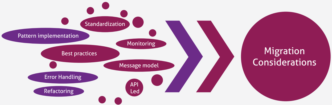
Migration Consideration
