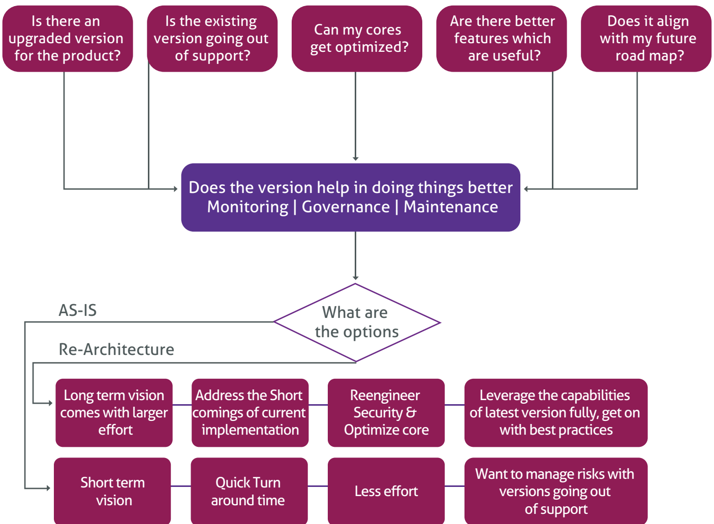
Decision Process
